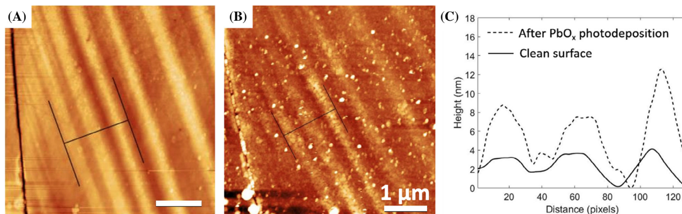
FIGURE 5 Atomic force microscopy (AFM) topography of a grain (A) before and (B) after photodeposition of \text{PbO}_x at 85^\circ\text{C} . The topography profiles of the same three domains in both are shown in (C). The profiles are averaged over 128 pixels.
