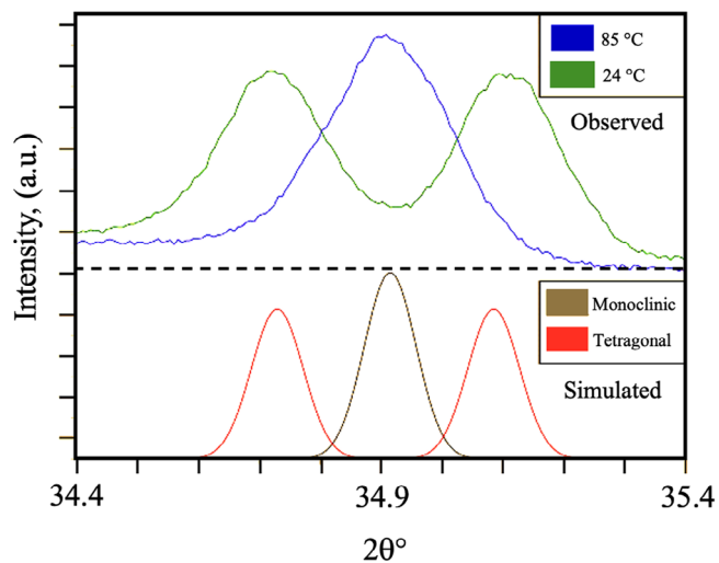
FIGURE 3 (A) X-ray diffraction (XRD) patterns of the x = 0.08 sample of (\text{Bi}_{1-0.5x}\text{Na}_{0.5x}(\text{V}_{1-x}\text{Mo}_x))\text{O}_4 on the hot plate at room temperature (in green) and at 85°C. (B) Simulated XRD patterns of x = 0.08 co-doped monoclinic (in black) and tetragonal (in pink) (\text{Bi}_{1-0.5x}\text{Na}_{0.5x}(\text{V}_{1-x}\text{Mo}_x))\text{O}_4 . The lattice parameters were obtained. 22
