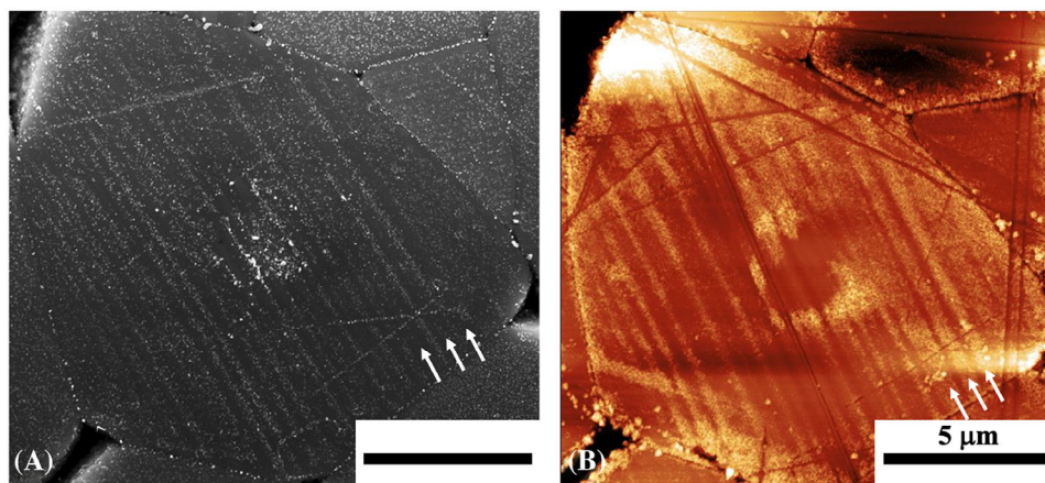
FIGURE 6 (A) Scanning electron microscopy (SEM) image of the surface after the photoreduction of Ag at room temperature. (B) Topographic atomic force microscopy (AFM) image after the photoanodic oxidation of \text{Mn}^{2+} at 85^\circ\text{C} .
