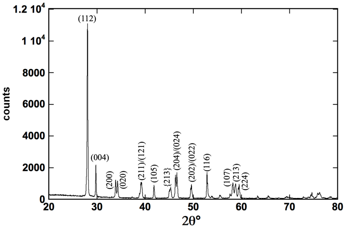
Figure S1. X-ray diffraction pattern of the Na, Mo co-doped sample, (Bi 1-0.5x Na 0.5x )(V 1-x Mo x )O 4 , x = 0.08.
