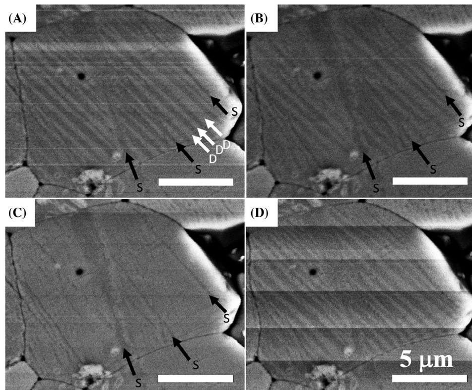
FIGURE 2 Hot-stage scanning electron microscopy (SEM) images of grain in x = 0.08 sample of (\text{Bi}_{1-0.5x}\text{Na}_{0.5x}\text{V}_{1-x}\text{Mo}_x)\text{O}_4 at different temperatures. (A) 40°C, (B) 55°C, (C) 70°C, and (D) after cooling back to 40°C. S denotes scratches and D denotes domains in the images.
