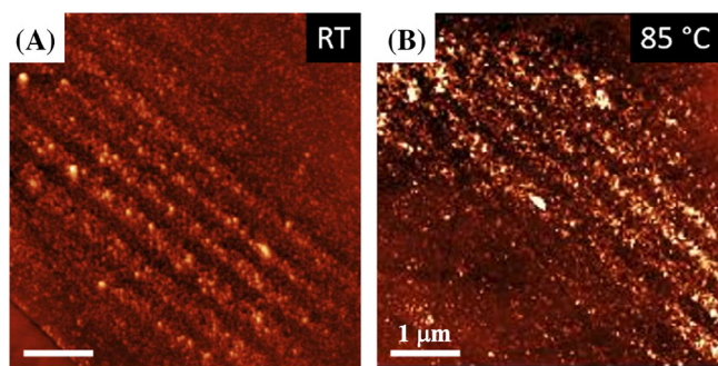
FIGURE 4 Atomic force microscopy (AFM) topography after photodeposition of \text{MnO}_x at (A) room temperature (RT) and (B) at 85^\circ\text{C} . Dark-to-light vertical scales: (A) 32 nm. (B) 14 nm.
