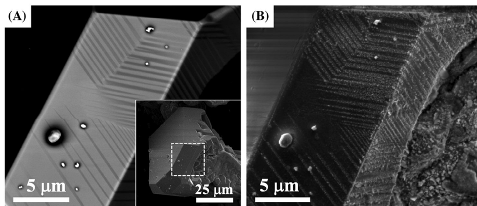
FIGURE 8 (A) Backscattered electron (BSE) image of two facets of a hydrothermally-grown \text{BiVO}_4 crystal. The entire crystal is shown in the inset. The BSE image is of the area inside the dashed line. (B) SE image of the same two facets after photodeposition of \text{Ag}^+ .
