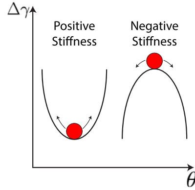
Fig. A.13. A schematic illustration of Eq. (A.6). The stiffness corresponds to the local curvature of the \Delta\gamma - \theta diagram.
