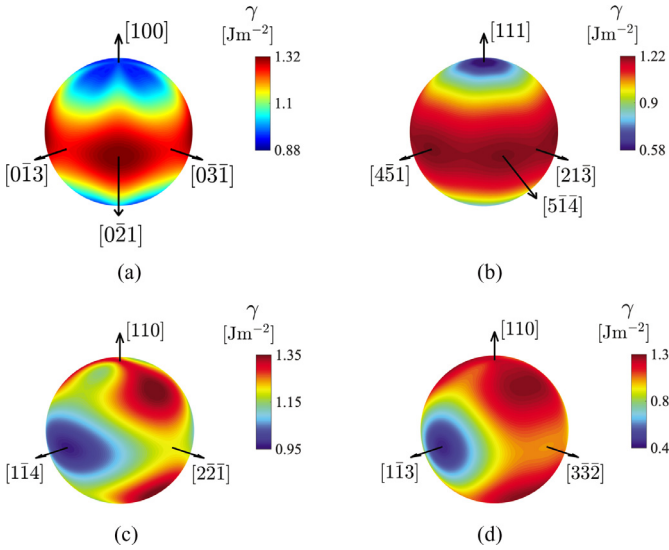
Fig. 3. The GB energy as a function of the plane normal \mathbf{n} for (a) \Sigma 5 , (b) \Sigma 7 , (c) \Sigma 9 , and (d) \Sigma 11 GBs. Here, \mathbf{n} = \mathbf{n}(\theta, \phi) , refer to Fig. 1(b) for the spherical angle convention used in this work. The polar and azimuthal angles are respectively measured from: [100] and [0\bar{1}3] for \Sigma 5 ; [111] and [4\bar{5}1] for \Sigma 7 ; [110] and [1\bar{1}4] for \Sigma 9 ; and [110] and [1\bar{1}3] for \Sigma 11 GBs.
