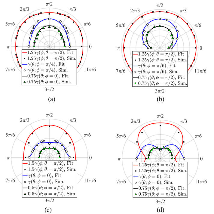
Fig. 4. Representative slices from the GB energy surfaces shown in Fig. 3 for (a) \Sigma 5 , (b) \Sigma 7 , (c) \Sigma 9 , and (d) \Sigma 11 GBs in Ni. The plots show the atomistic simulation data (markers) from the study by Olmsted et al. [16] and the fits (solid lines) using Eq. (7).
