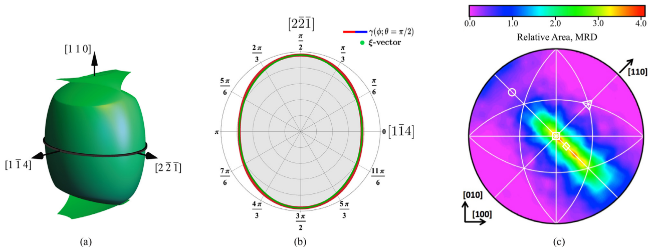
Fig. 10. For the \Sigma 9 GB in Ni, (a) a plot of the Cahn-Hoffman \xi -vector. (b) A line scan along \theta = \pi/2 depicting the \xi -vector (green) and GB energy, which is colored by the stiffness \gamma + \gamma_{\phi\phi} , where red (blue) denote positive (negative) stiffness values. (c) Experimentally-determined relative areas of GB planes, shown in stereographic projection along the [001] direction. The orientation of the [110] misorientation axis is shown by the arrow, and the [001] direction is at the position of the white square. The [111] direction is denoted by the white triangle. The white diamond and circle mark, respectively, the orientation of the (\bar{1}\bar{1}4)||(\bar{1}\bar{1}4) and (\bar{2}\bar{2}1)||(\bar{2}\bar{2}1) symmetric tilt GBs (For interpretation of the references to color in this figure legend, the reader is referred to the web version of this article.)
