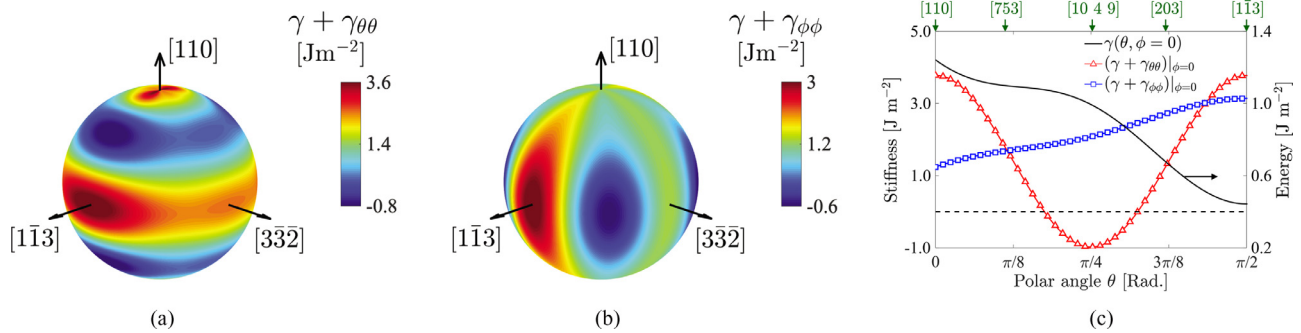
Fig. 11. For the \Sigma 11 GB in Ni, principal stiffness values (a) \gamma + \gamma_{\theta\theta} and (b) \gamma + \gamma_{\phi\phi} . (c) A line scan along \phi = 0 depicting the polar angle dependency of the GB energy and principal stiffness values.
